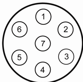
ISO 1724 7-pol
